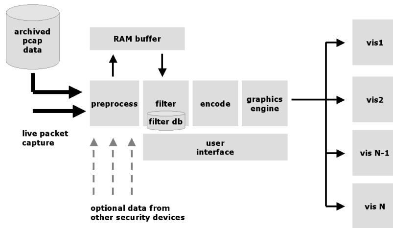
Figure 5: System Architecture. Network traffic is collected through packet capture or replayed from forensic pcap files. The system stores complete packets, both headers and payloads, in a RAM buffer. The user interacts with the user interface and the resulting data is pulled from the buffer and sent to the graphics engine for display using a number of visualizations. Additional information may be provided by devices such as firewalls and intrusion detection systems and used to assist encoding, filtering and semantic zooming.
