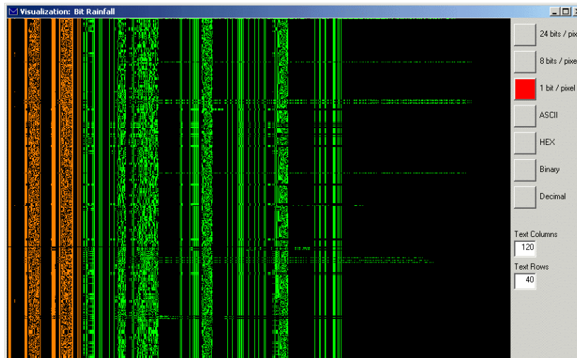
Figure 1: Binary Rainfall Visualization of Defcon 11 “Capture the Flag” Network Traffic. One packet is plotted per horizontal line. In this level of zoom, each pixel represents one bit of network traffic. Network layer protocol headers are encoded in orange and the encapsulated IP payload is encoded in green. This visualization allows analysts to readily compare approximately 600-1000+ packets per screen.
